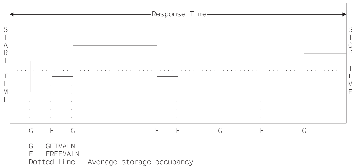
Figure 10. Storage occupancy
