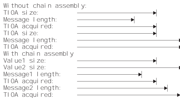
Figure 14. Message length and terminal input/output area length
