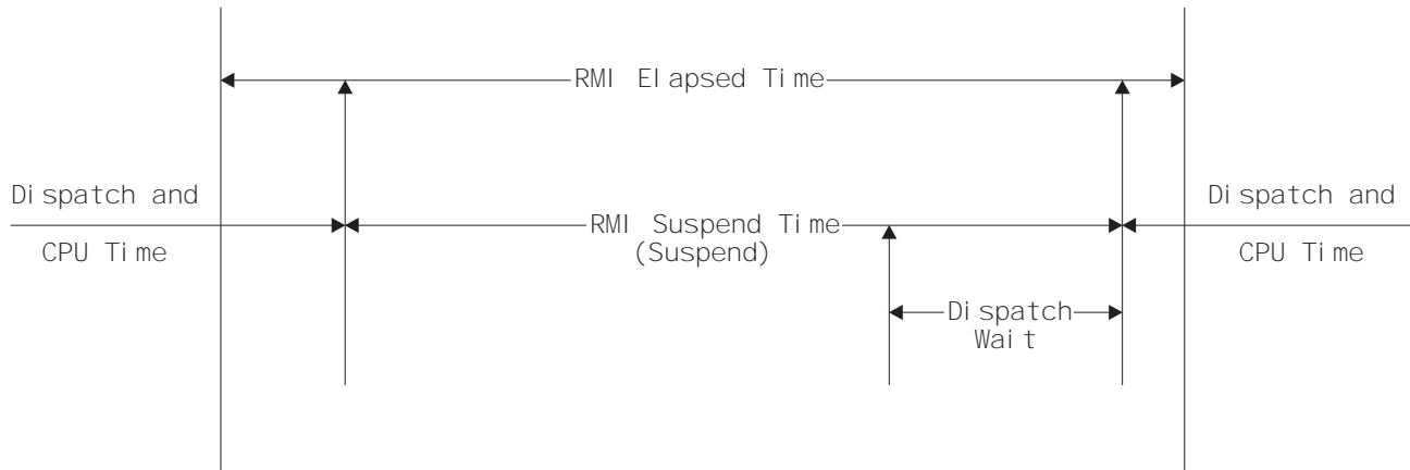
Figure 9. RMI elapsed and suspend time
