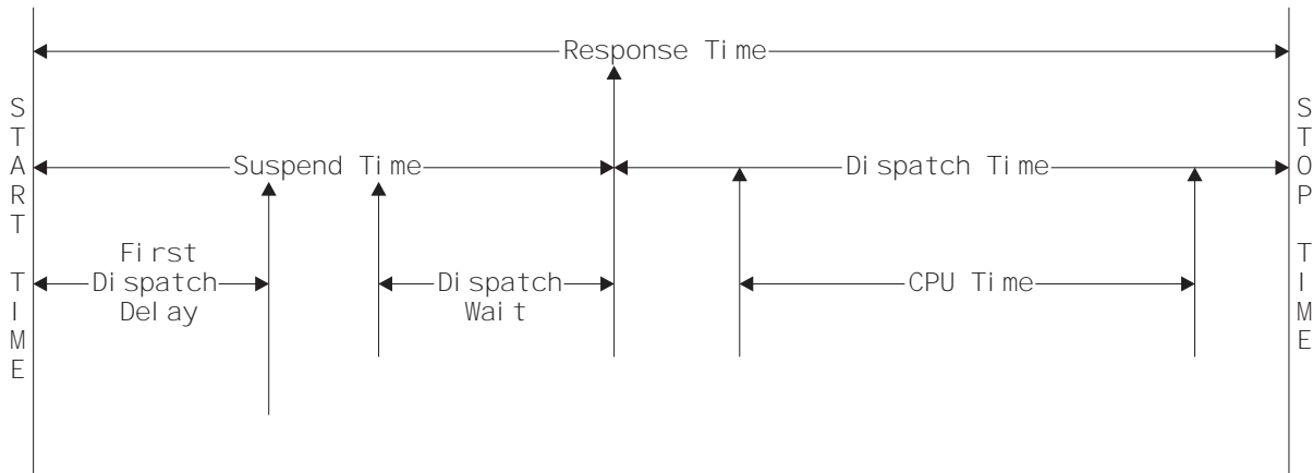
Figure 5. Response time relationships
